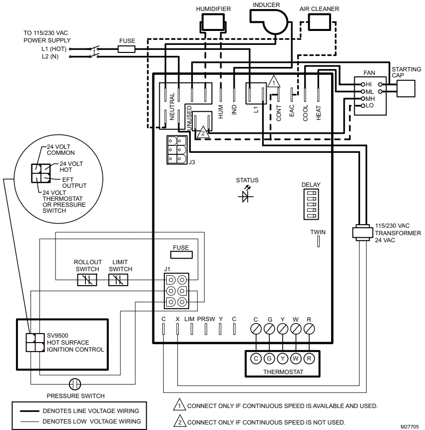
Fig. 2. Typical ST9120U,B wiring connections in ST9120 system with SV9500/SV9501 SmartValve™ Control.
