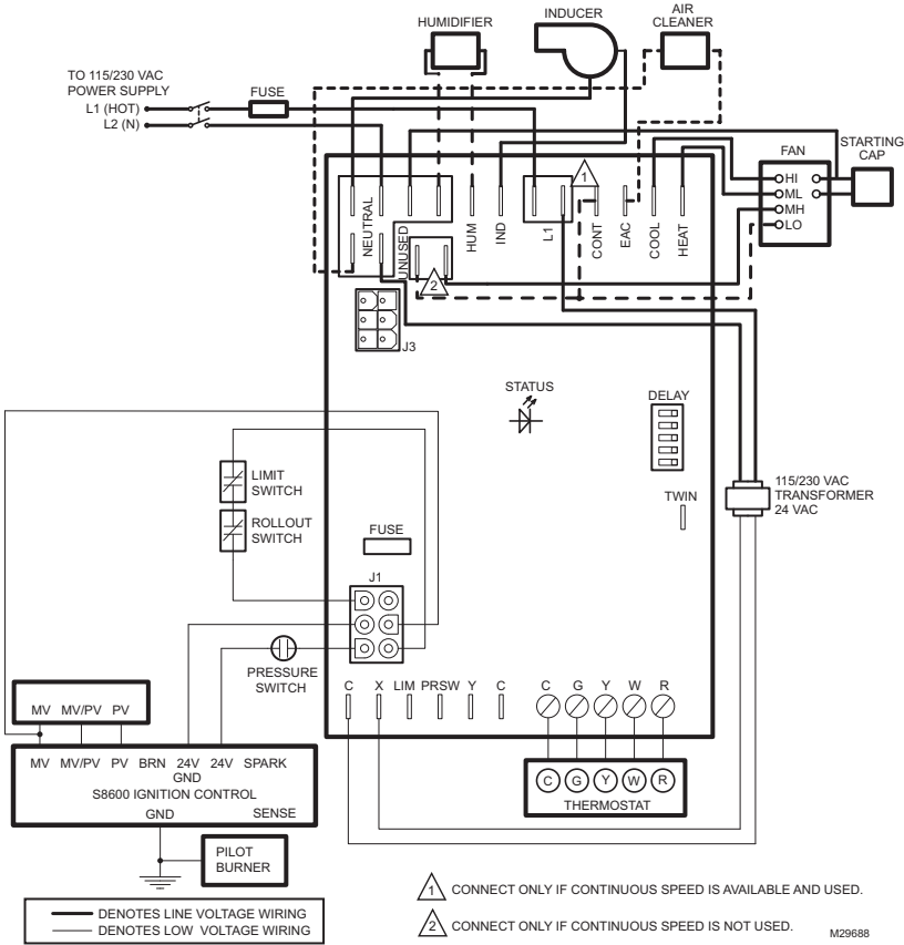
Fig. 1. Typical ST9120U,B wiring connections in ST9120 system with S8600 Intermittent Pilot Ignition Control.
