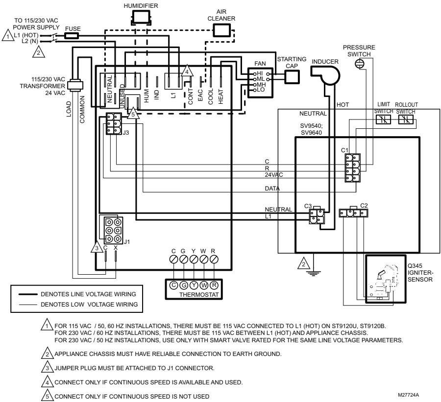
Fig. 6. Typical ST9120U,B wiring connections in ST9160 system with SV9540/SV9640 SmartValve™ Control.
