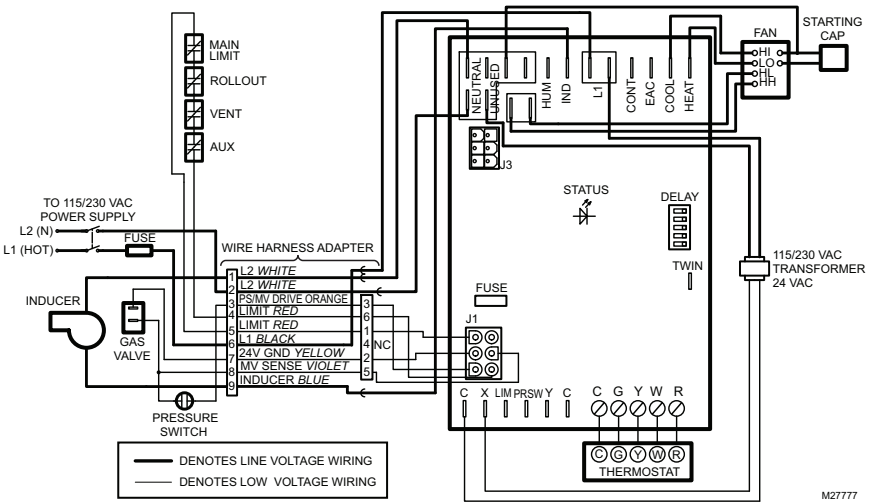
Fig. 3. Typical ST9120U,B wiring connections in ST9101 system.
